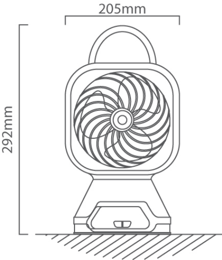
F84 CAD DIAGRAM
